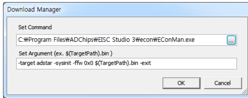
[ Download Option ]
