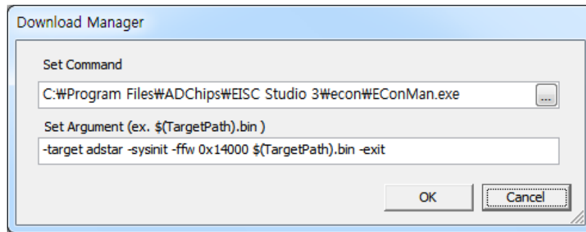
[ download option ]
