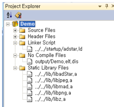
[ Linker Script ]
