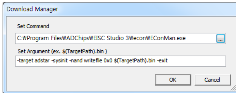
[ Download Option ]
