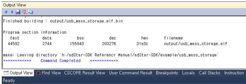
[ Output View ]
