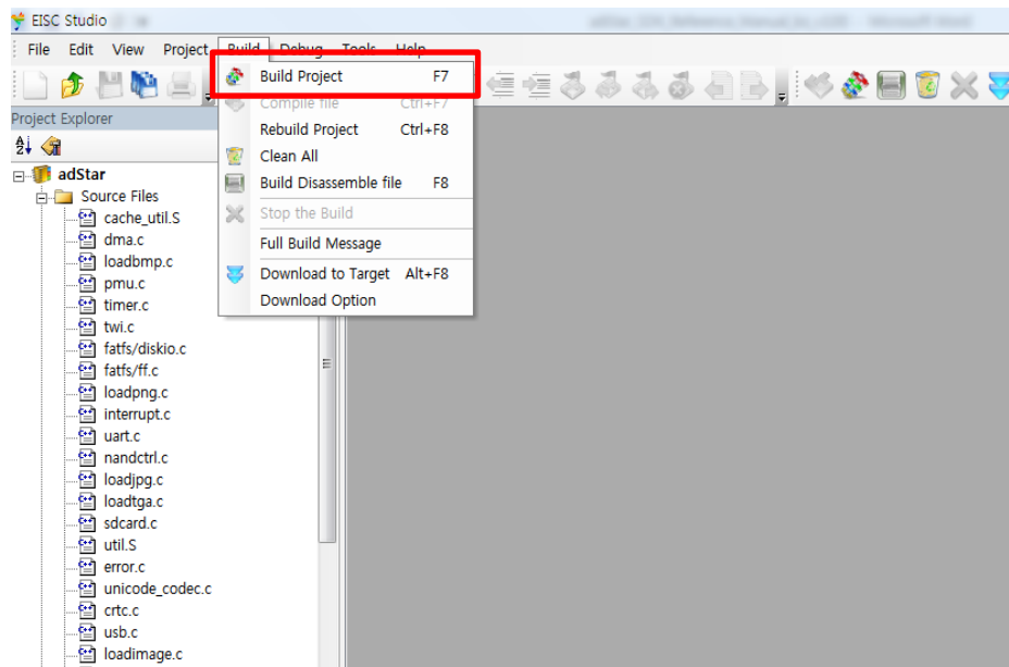
[ Build Project ]
