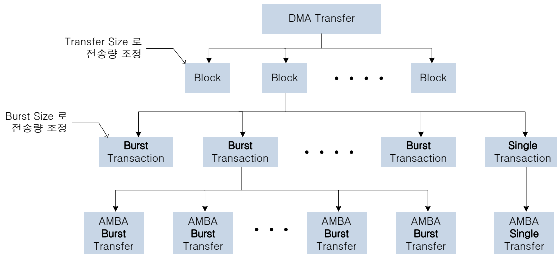
Figure 9-4 Multi Block Transfer
