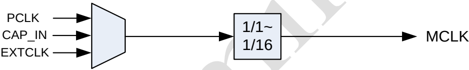
Figure 22-3 I2S Pre-Scaler
