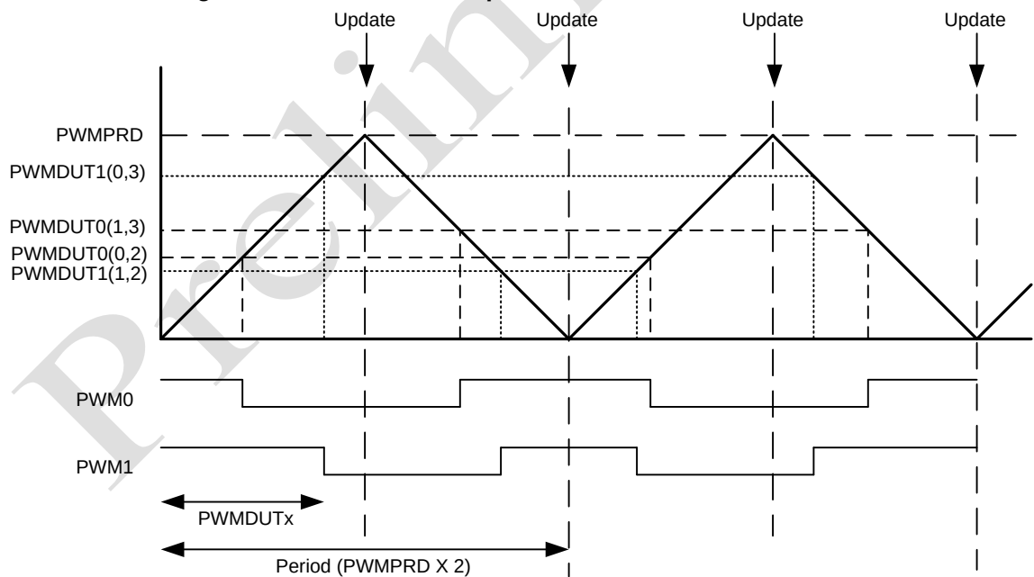
Figure 24-4 Center Aligned PWM with Double Update
