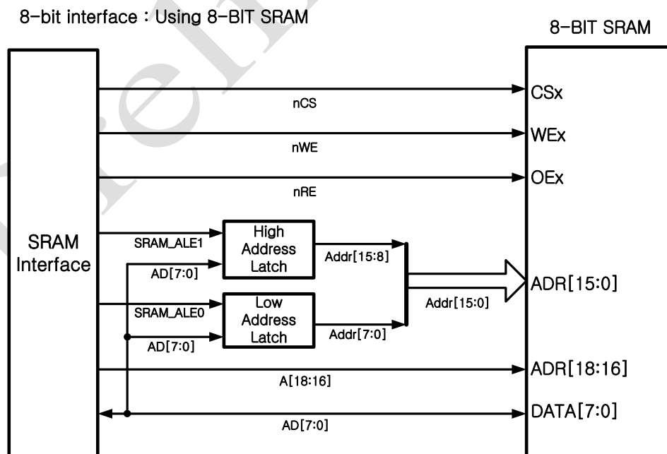
Figure 12-2 Connection 8-bit SRAM Memory
