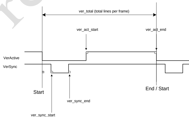
Figure 24-6 Vertical Timing
