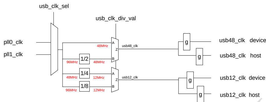
Figure 4-9 USB Clock
