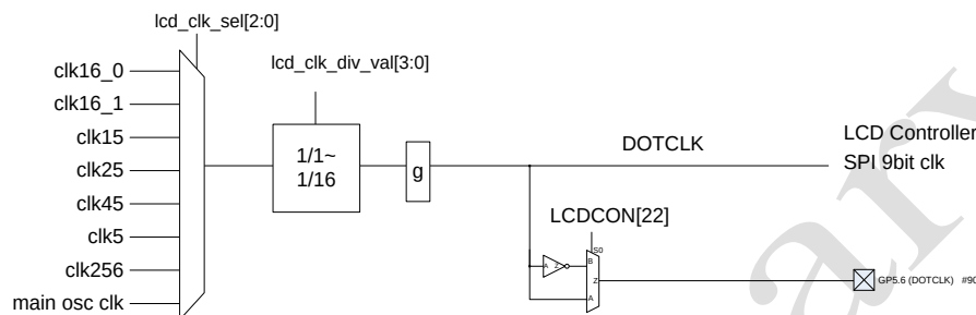
Figure 24-2 LCD Clock
