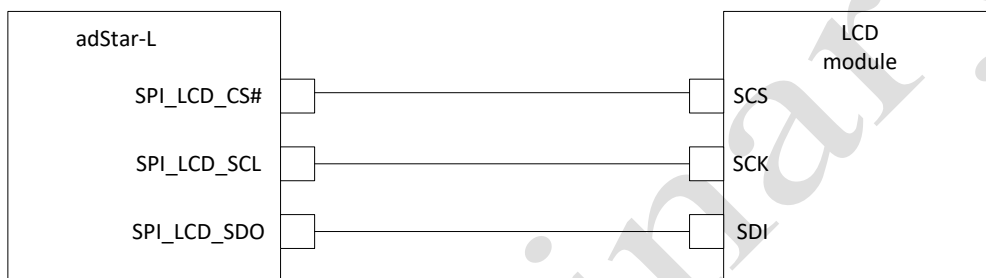
Figure 19-3 9bit mode pin connection
