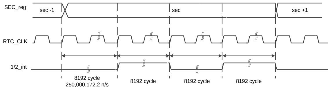
Figure 12-5 1/2 Interrupt Operation
