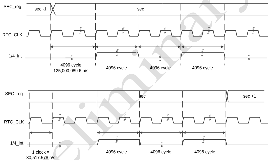
Figure 12-6 1/4 Interrupt Operation
