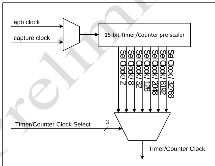
Figure 11-1 Pre-scaler Block Diagram
