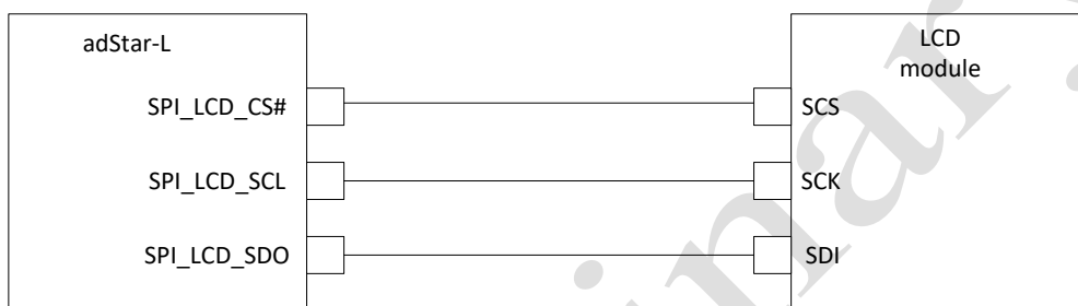
Figure 19-3 9bit mode pin connection
