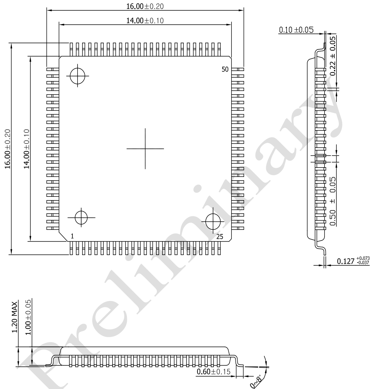
Figure 29-1 Package Dimension
