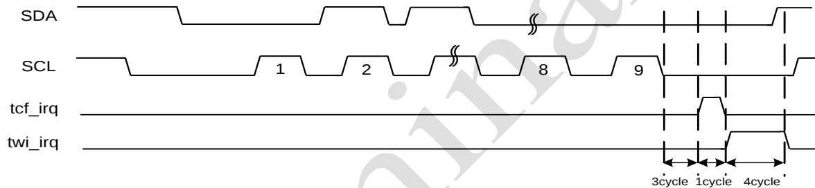
Figure 21-13 Tcf interrupt wave form
